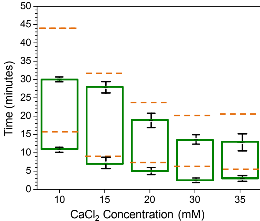
Figure 21. B. cereus settling time versus CaCl 2 concentration. Results represent the time at which flocs formed in the columns (the bottom of the box) and the time that they finished their decent to the bottom of the column (top of the box). The dotted lines represent the control begin and end time. Columns contained 10 8 cells/mL suspended in hard water (HW) treated with a range of CaCl 2 concentrations both alone and with the addition of 2 ppm Non-Gelling Extract (NE)
