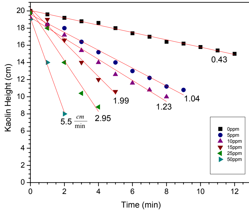
Figure 14. Truncated kaolin plot with linear curve fit slopes. Resulting slope represents the settling rate of the kaolin in cm/min.
